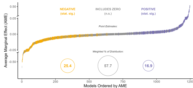
Fig. 1. Broad variation in the findings from 73 teams testing the same hypothesis with the same data. The distribution of estimated AMEs across all converged models ( n = 1,253 , point estimates shown as hash marks) includes results that are negative (yellow; in the direction predicted by the given hypothesis the teams were testing), not different from zero (gray), or positive (blue) using a 95% CI. AME are xy -standardized. The y axis contains two scaling breaks at \pm 0.05 . Numbers inside circles represent the percentages of the distribution of each outcome inversely weighted by the number of models per team.
